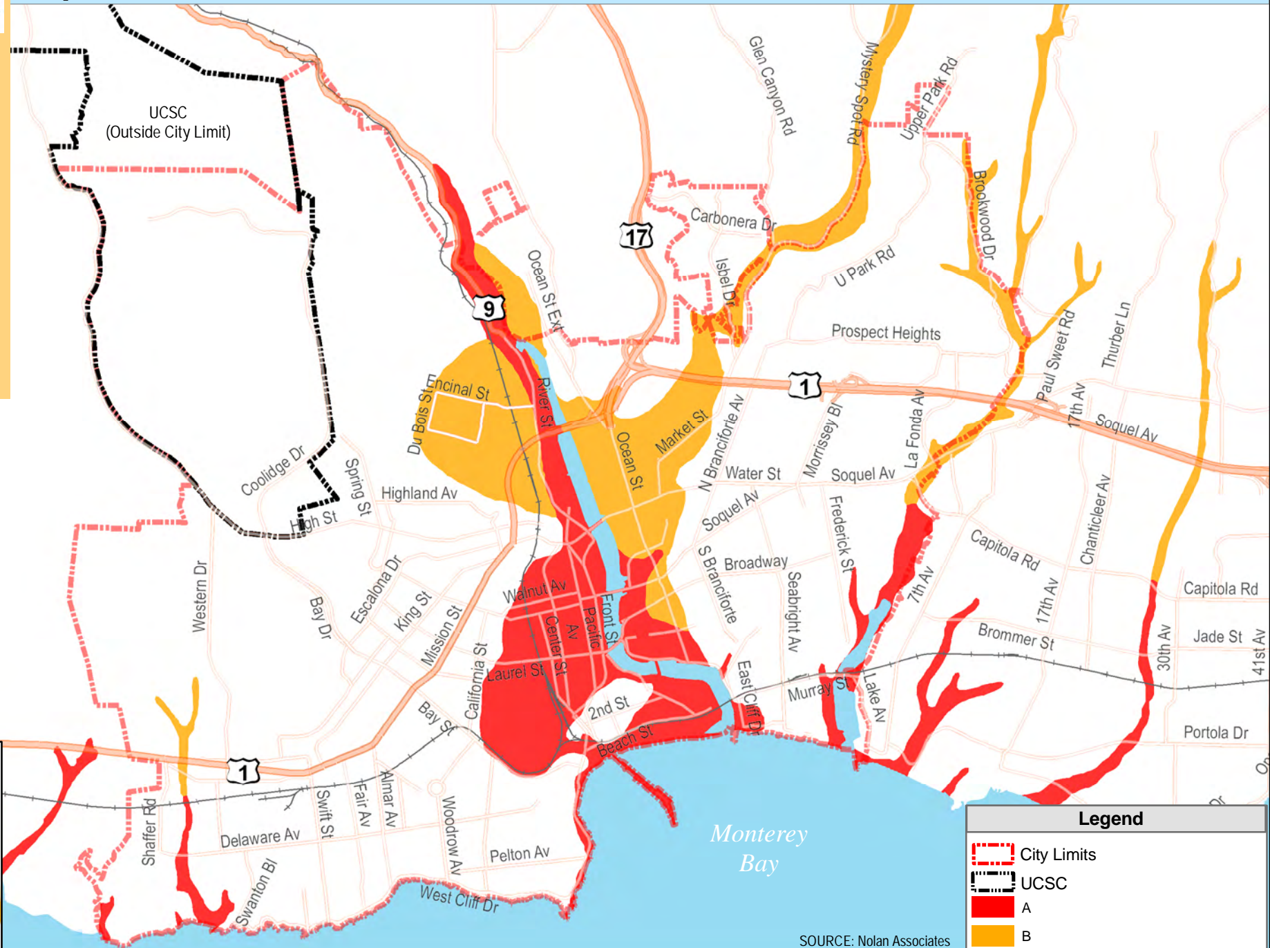
Figure 4.10-4 Liquefaction Hazards
