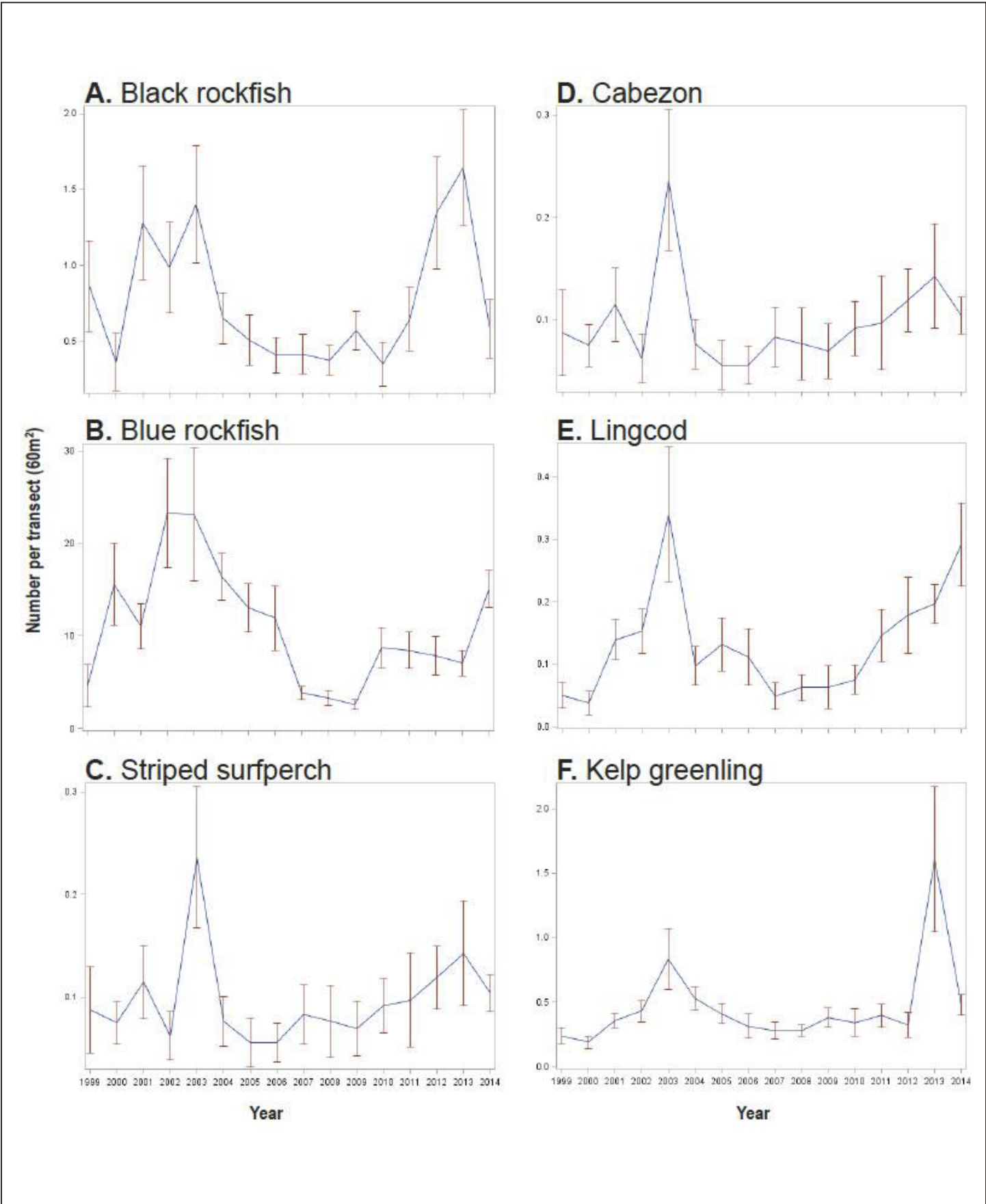
FIGURE 4.2-2 Annual Mean Abundance Estimates from Monitoring Sites around Monterey and Pt. Lobos for Groundfish Species, 1999-2014 (PFMC 2016)
